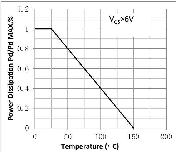
Fig.3 Power Dissipation
