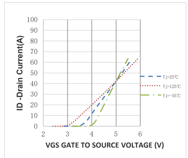
Figure 10. Transfer Characteristics
