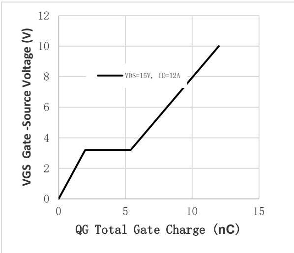
Fig.1 Gate-Charge Characteristics
