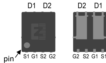
DFN5*6
