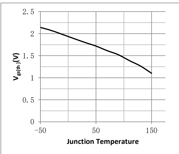
Fig.5 Threshold Voltage Vgs(th) V.S Junction Temperature
