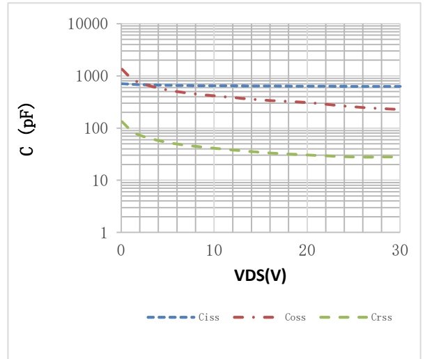
Fig.2 Capacitance Characteristics
